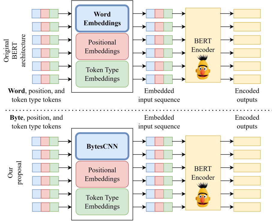
Figure 2: Illustration of the replacement of the transformer word embedding layer with the aligned BytesCNN.
