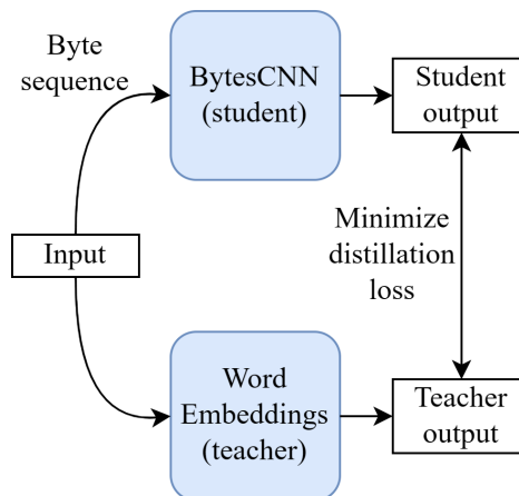
Figure 1: Embedding alignment framework.
